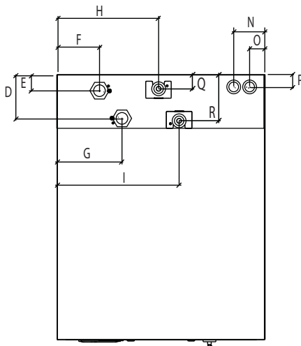
WRL-E 050 - 070 - 080 (AIR COOLED CONDENSED REMOTE / SYSTEM SIDE)
