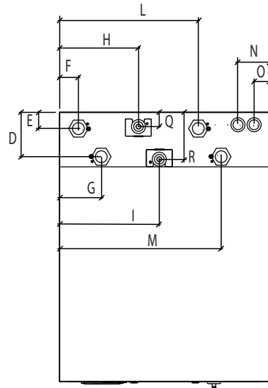
WRL-E 050 - 070 - 080 (AIR COOLED CONDENSED REMOTE / SYSTEM SIDE / DESUPERHEATER)
