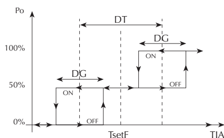
Termostato Freddo a due gradini Two Steps Cooling Thermostat
