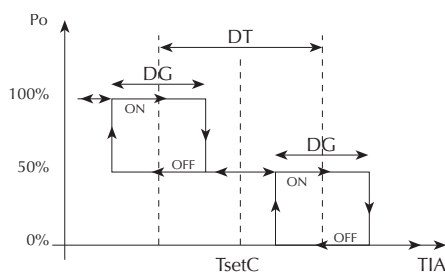
Termostato Caldo a due gradini Two Steps Heating Thermostat
