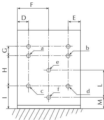
Vista posteriore con attacchi idraulici Rear view with water connections
