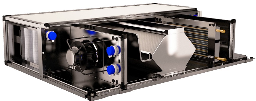
Fans of supply and extract of plug-fan-type with synchronous motor with electronic control permanent magnetos (EC)
